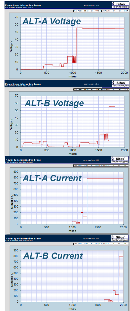
802.3bt Dual Class 5, 90W Power-Up
